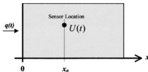
Figure A1. Schematic of the 1D heat conduction problem where the temperature measurements from a depth x_a are used to estimate the surface heat flux q(t) .
